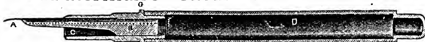
Sectional View. References—A, Gold Pen; B, Feed Bar; C, Point-section; D, Barrel; G, Knurl.
